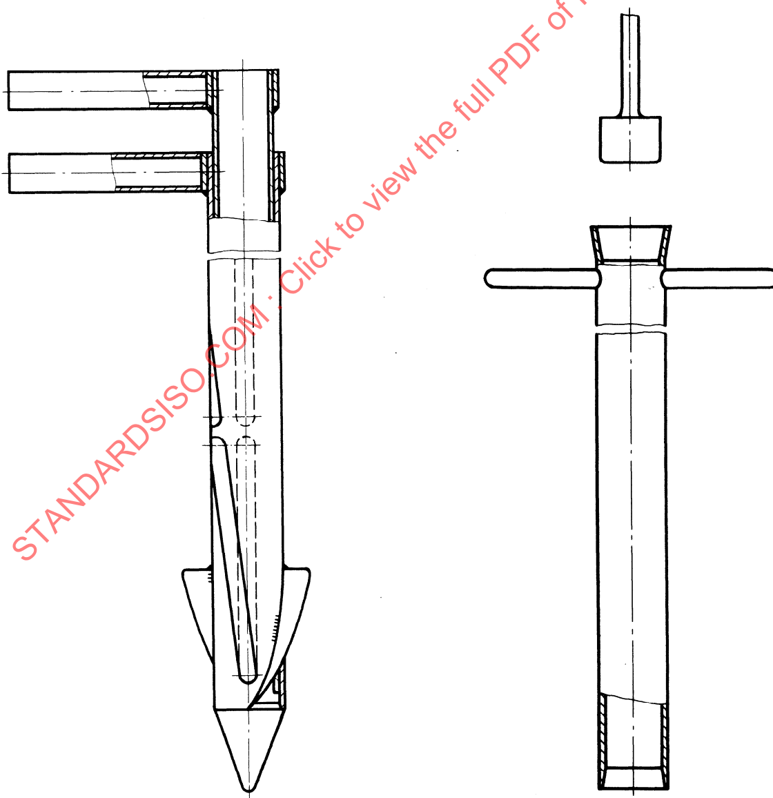
Figure 4 — Examples of probes for increment sampling
