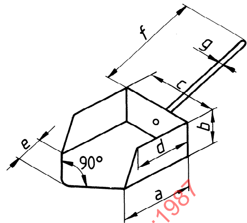
Figure 2 — A scoop for increment sampling
