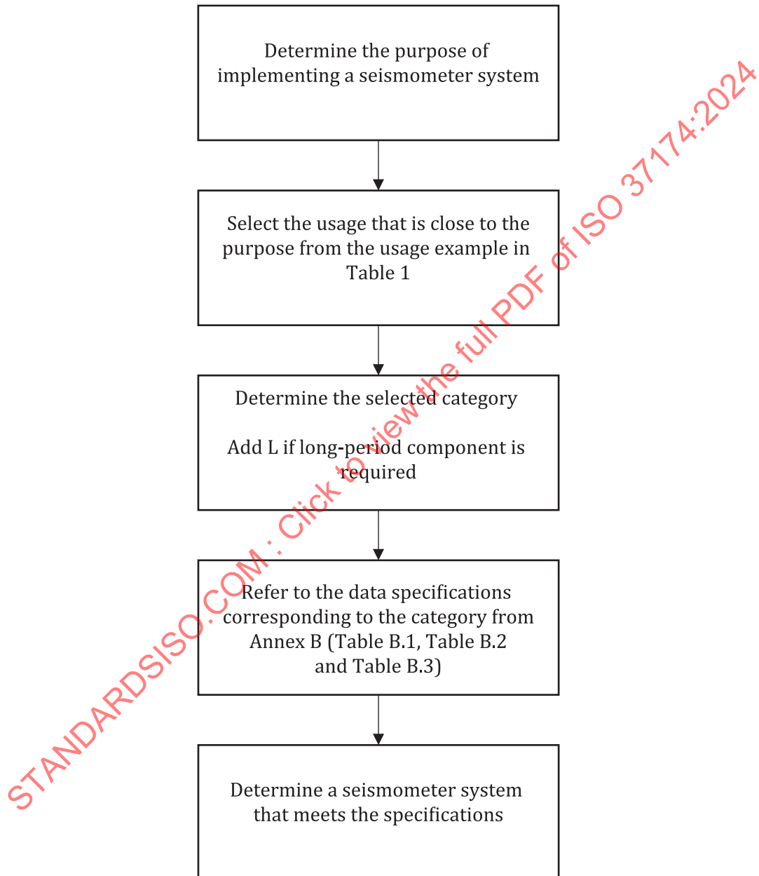
Figure A.1 — Flowchart for determining seismometer systems for specific purposes
