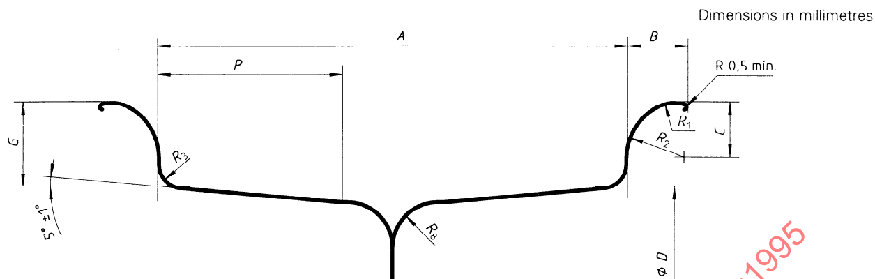
Figure A.1 — Tapered divided rims
