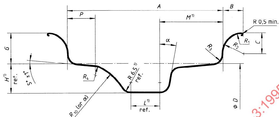
Figure A.2 — 5° drop-centre rims
