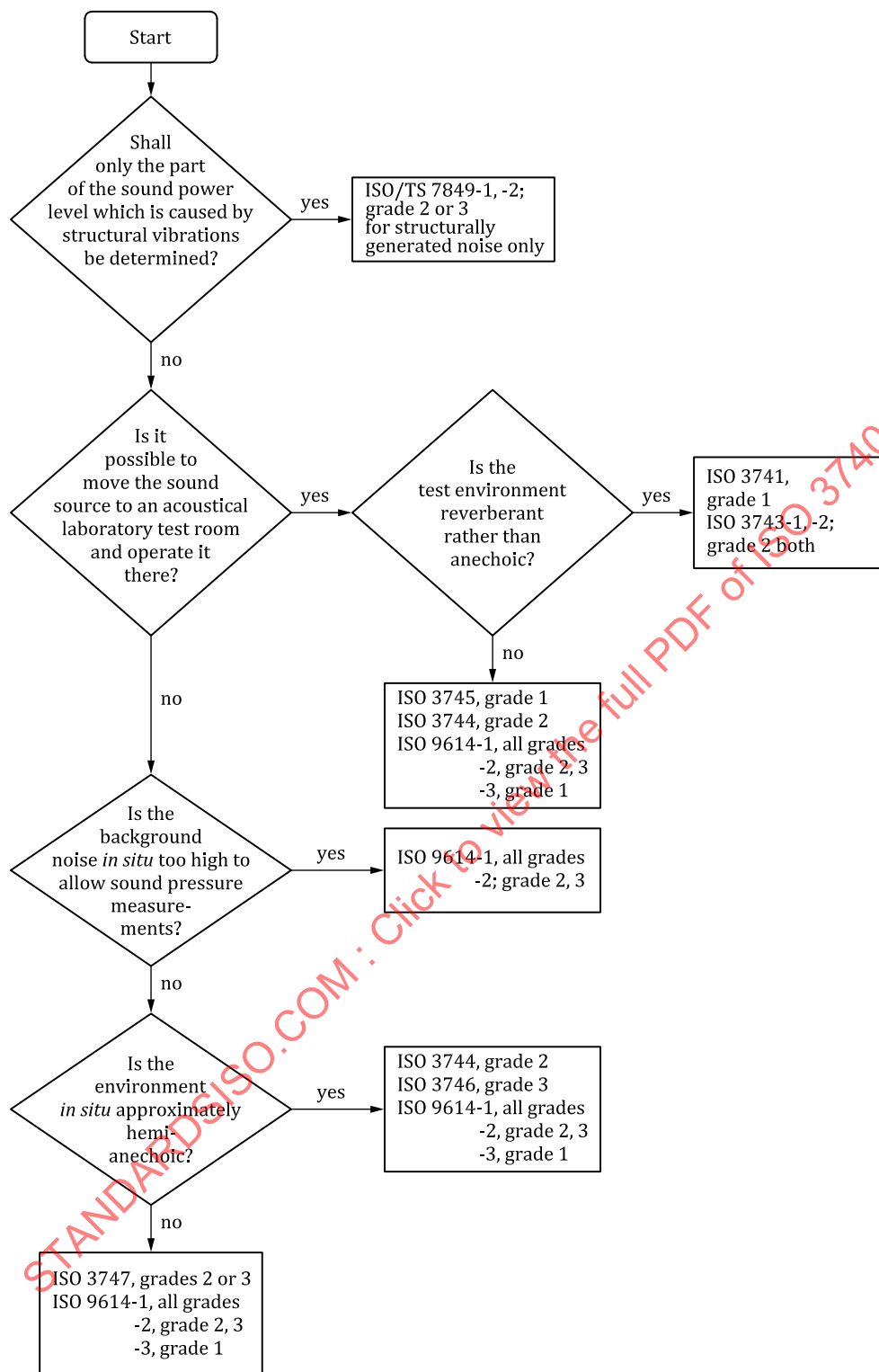
Figure 1 — Flowchart guiding the selection of appropriate International Standards for the determination of sound power levels
