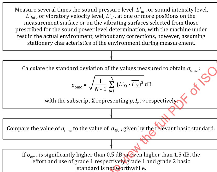
Figure C.1 — Flowchart to assist determining \sigma_{\text{omc}} , together with a guideline for the selection of the appropriate grade of accuracy
