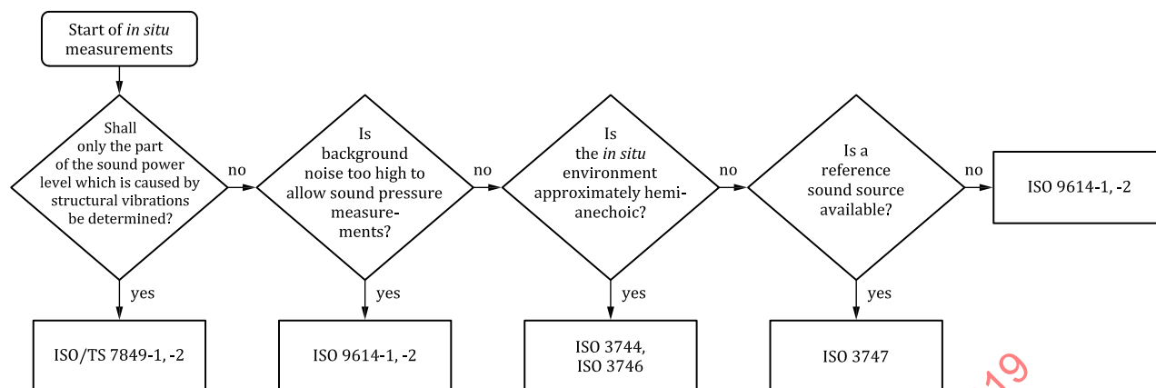
Figure 2 — Flowchart guiding the selection of International Standards for the determination of sound power levels appropriate for in situ measurements
