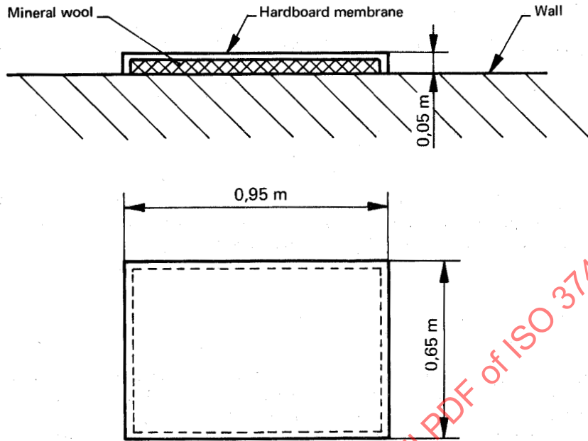
FIGURE 2 — Hardboard membrane absorber
