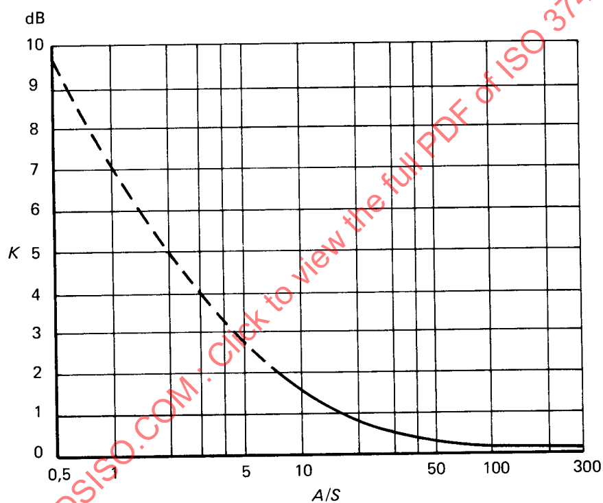
Figure 1 — Environmental correction K , in decibels
