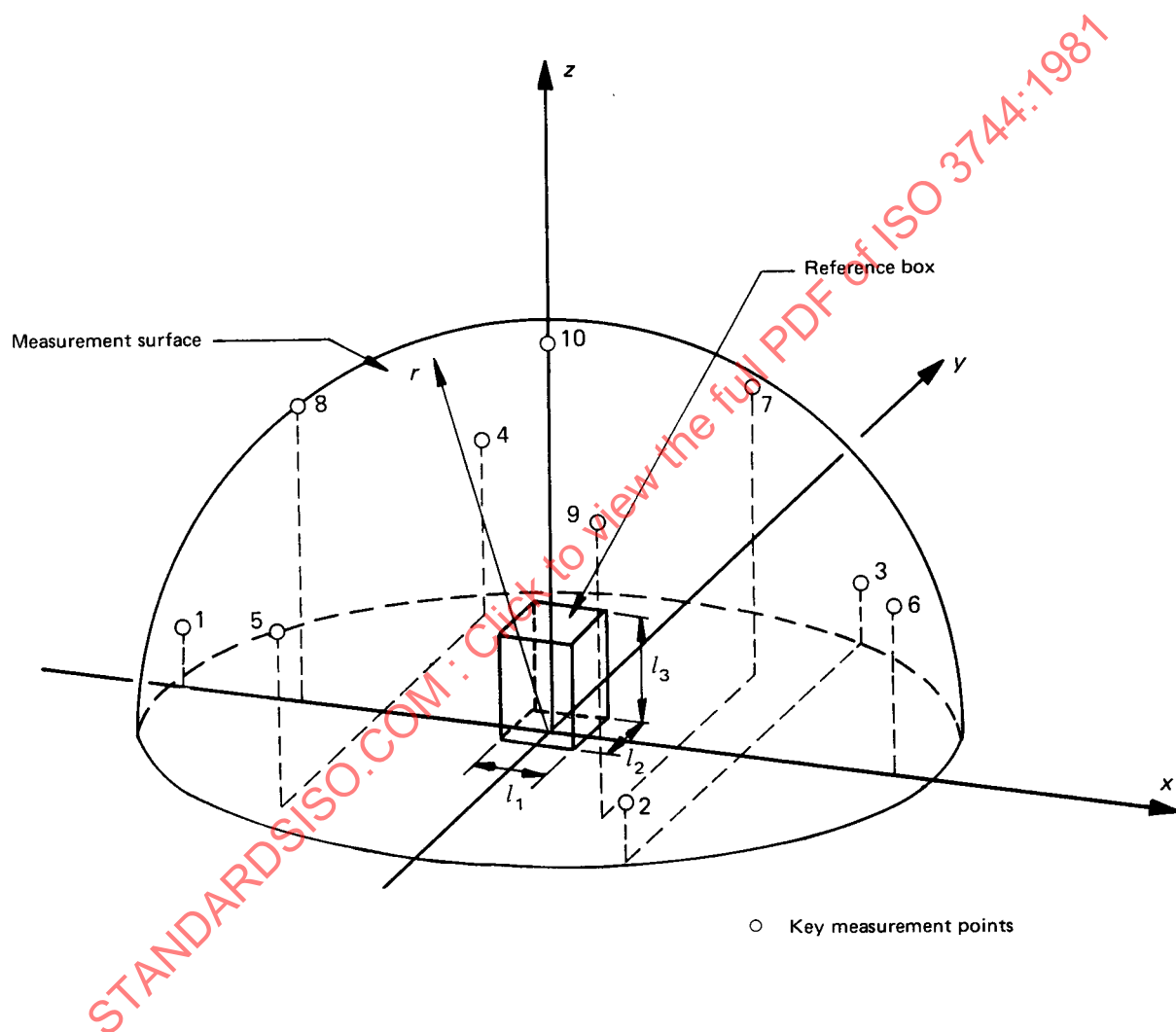
Figure 2 — Hemispherical measurement surface — Key measurement points
