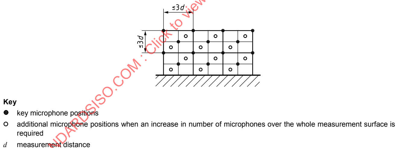
Figure C.2 — Additional microphone positions over the whole parallelepiped measurement surface consisting of rectangular partial areas
