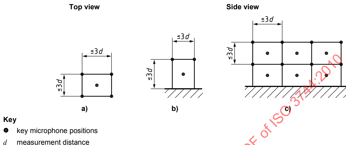
Figure C.1 — Key microphone positions on a parallelepiped measurement surface consisting of rectangular partial areas
