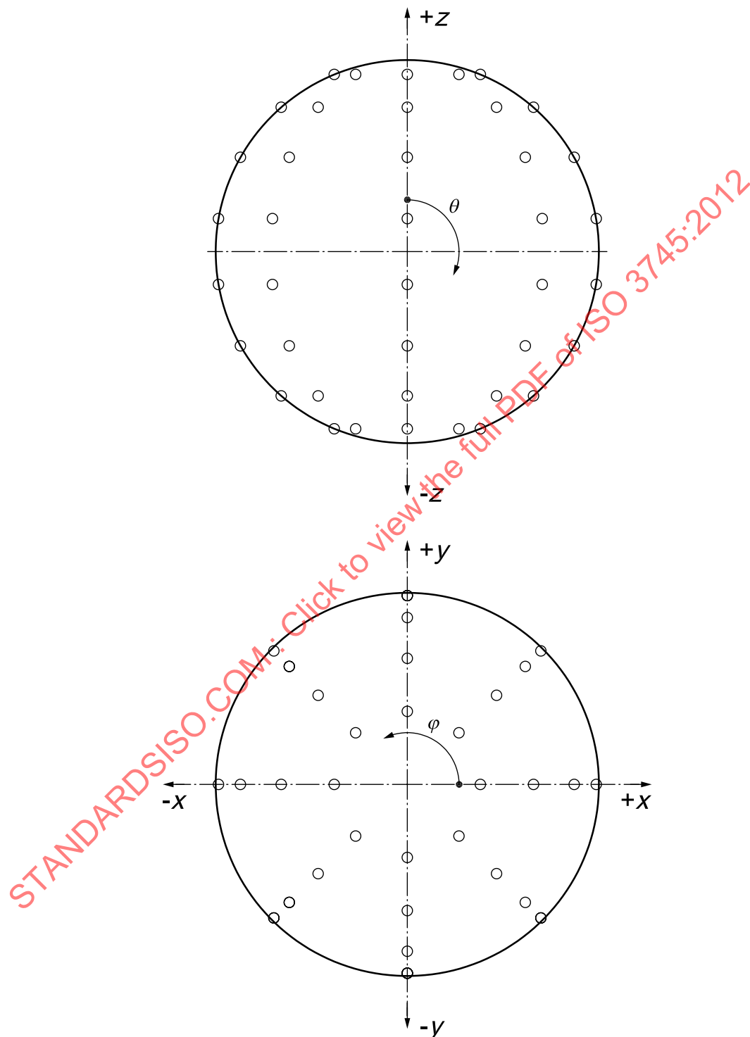
Figure A.1 — Microphone positions on the spherical surface for test sound source directivity measurements
