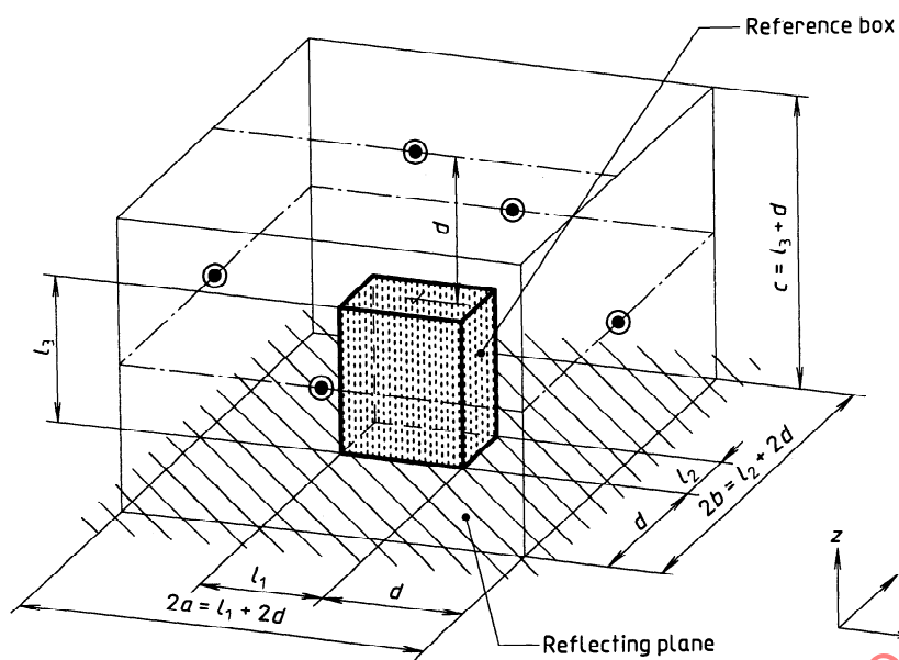
Figure C.2 — Example of a measurement surface and microphone positions for a small machine ( l_1 \leq d , l_2 \leq d , l_3 \leq 2d , where d is the measurement distance, normally 1 m)
