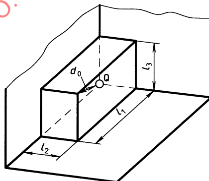
c) Reference box on three reflecting planes
