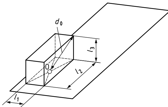
a) Reference box on one reflecting plane, d_0 = \sqrt{(l_1/2)^2 + (l_2/2)^2 + l_3^2}
