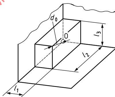
c) Reference box on three reflecting planes, d_0 = \sqrt{l_1^2 + l_2^2 + l_3^2}
