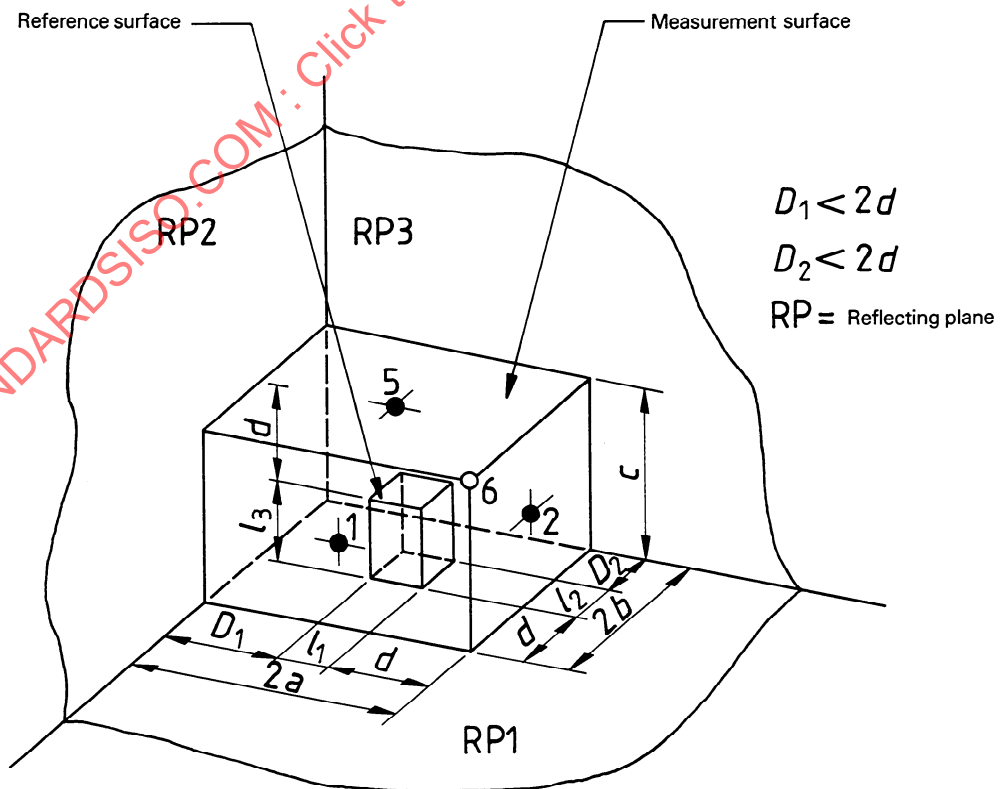
Figure 7 — Key (•) and additional (○) microphone positions for three-sided measurement surface
