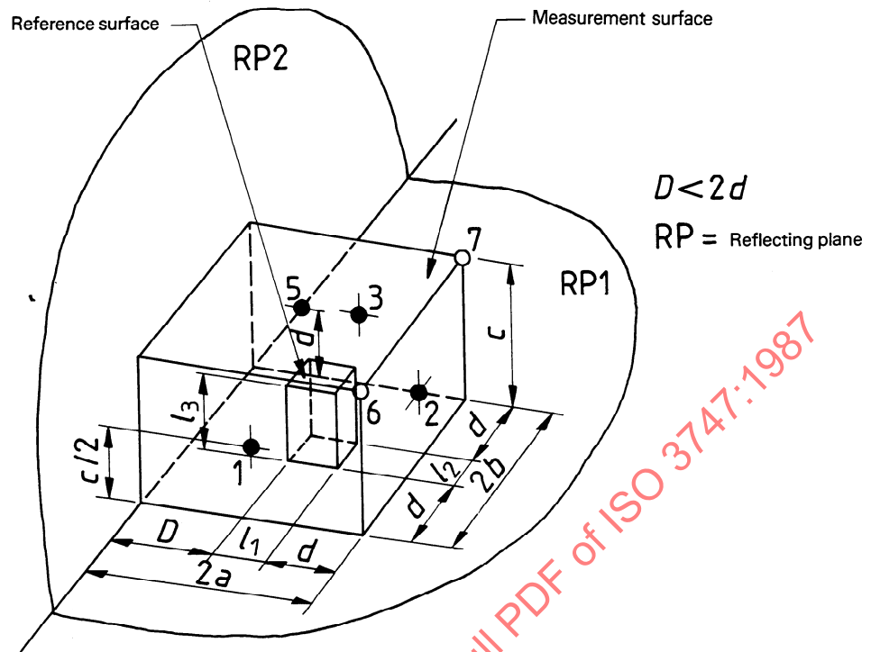
Figure 6 — Key (•) and additional (○) microphone positions for four-sided measurement surfaces
