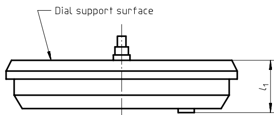
Figure 5 — Mechanical movement
