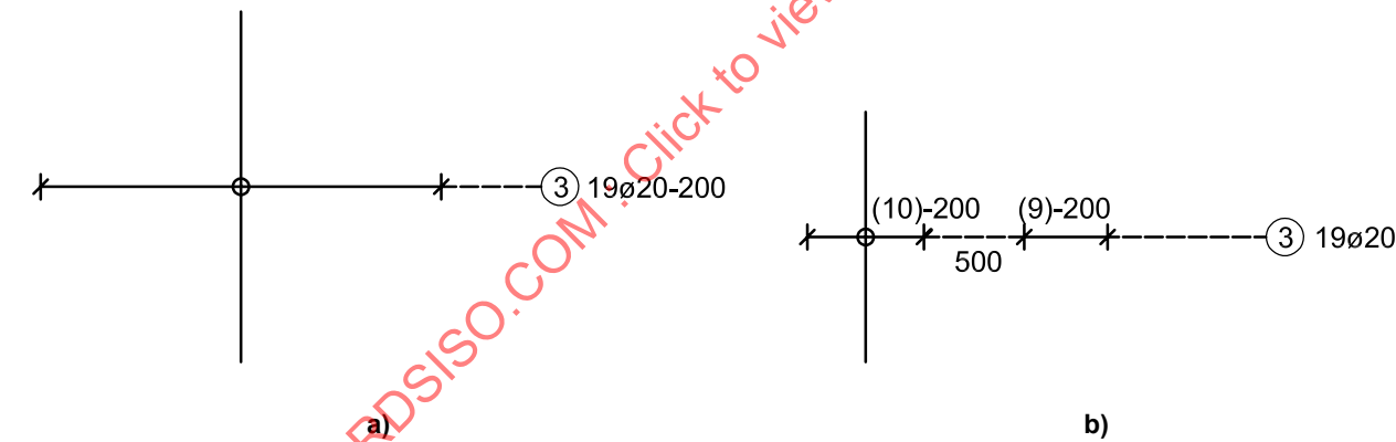
Figure 1 — Examples of bar markings (without options)
