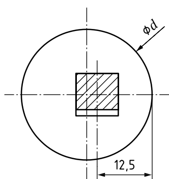
a) Where d \leq 25 mm
