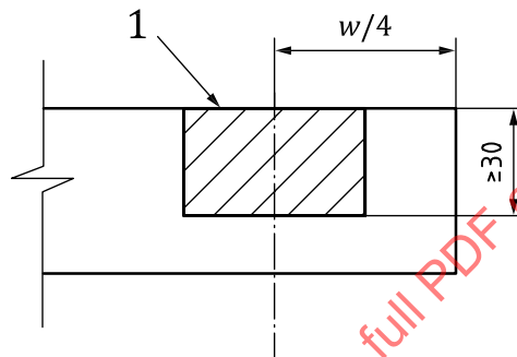
a) Full section test piece (preferred, see A.6.1 )
