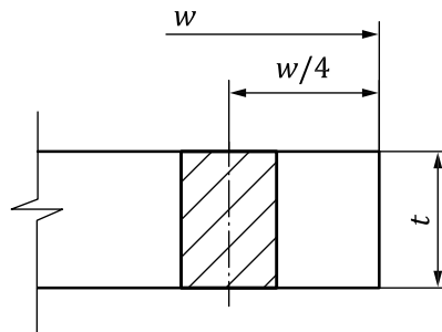
a) Full section test piece (preferred, see A.6.1 )
