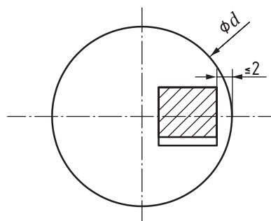
b) Where 25 \text{ mm} < d \leq 50 mm
