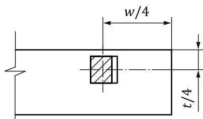
a) For all values of t
