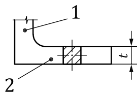
a) Full thickness test piece where t \leq 50 mm
