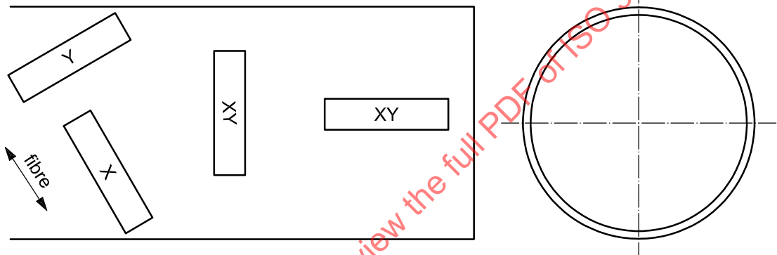
e) Thin-walled tube with helical grain flow
