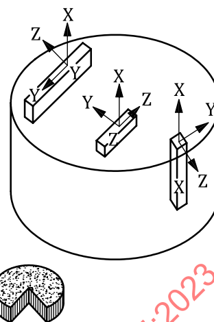
c) Cylinder — Axial grain flow, radial working direction
