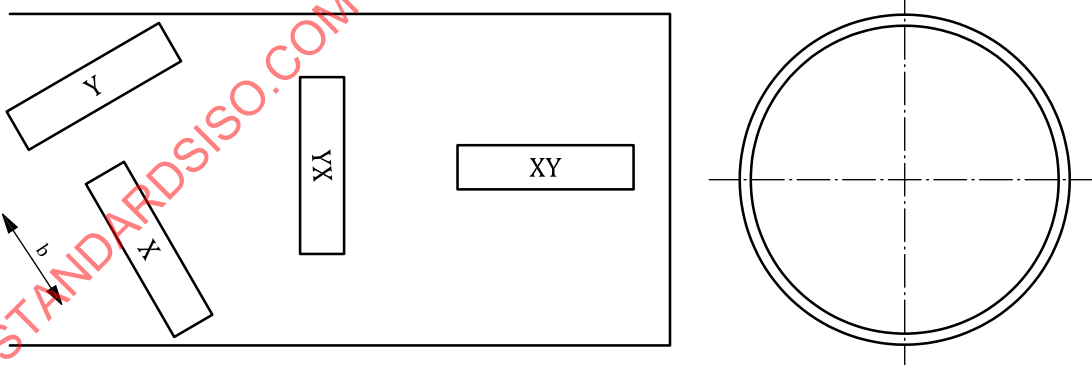
e) Thin-walled tube with helical grain flow
