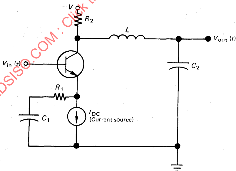
FIGURE 5 — Example of amplifier-differentiator
