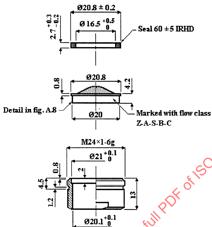
Figure A.6: Strainer type flow resistance with external thread M24 × 1 - 6g
