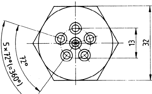
Figure A.4: Arrangement of the tubes for resistance R63
