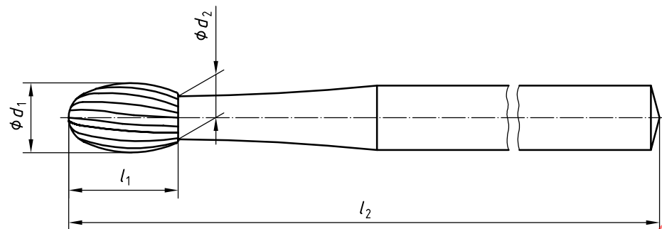
Figure 5 — Egg, steel finishing burs
