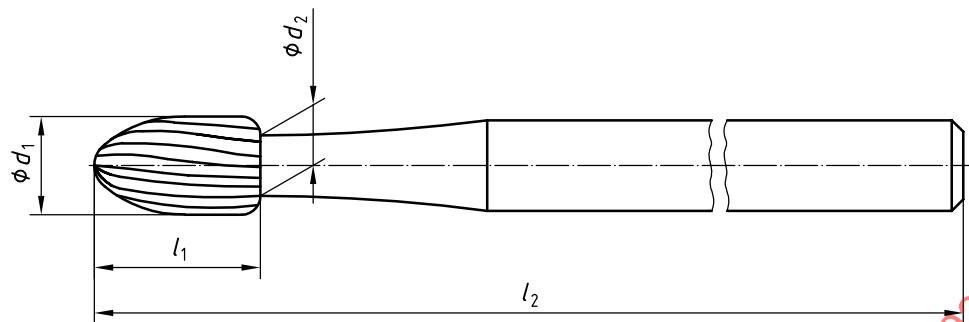
Figure 13 — Egg, carbide finishing burs
