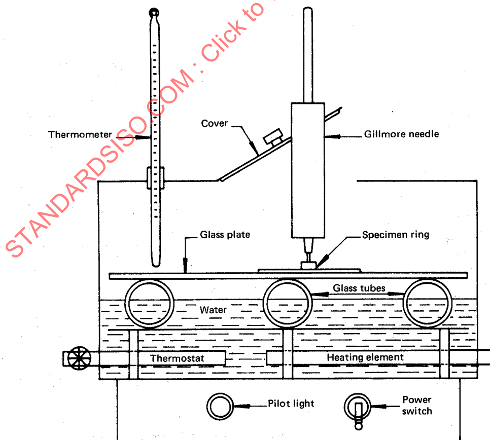
FIGURE 2 — Apparatus for determination of setting time at controlled temperature and humidity
