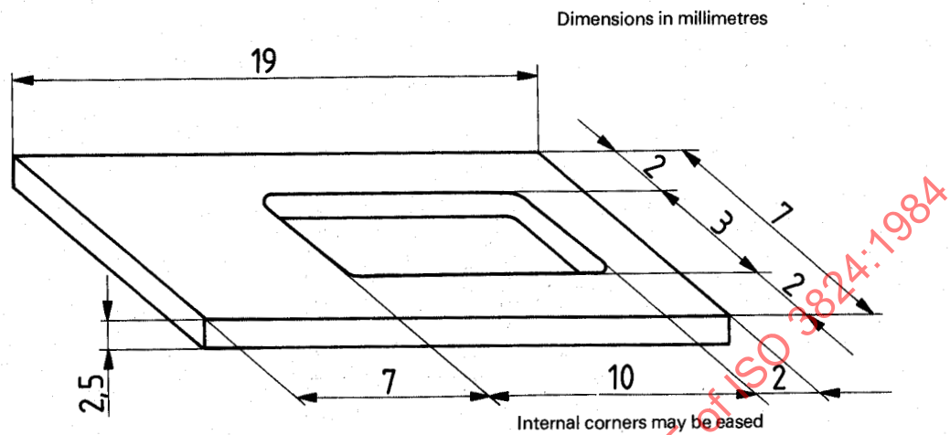
Figure 3 — Mould for use in determining the setting time
