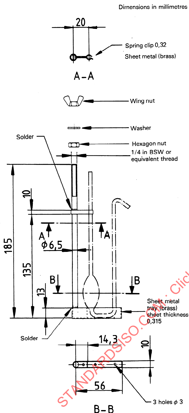
Figure 3 — A suitable design of holder for graduated bicapillary pyknometer
