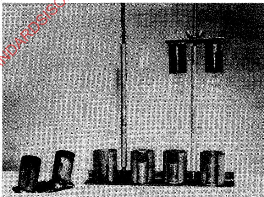
FIGURE 7 — Sulphonation flask holder and clamp for shaking machine
