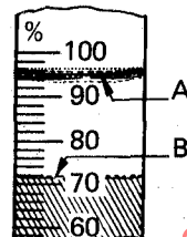
FIGURE 4 — Illustration of method for reading volume of unreacted hydrocarbon in sulphonation flask (see 7.5)
