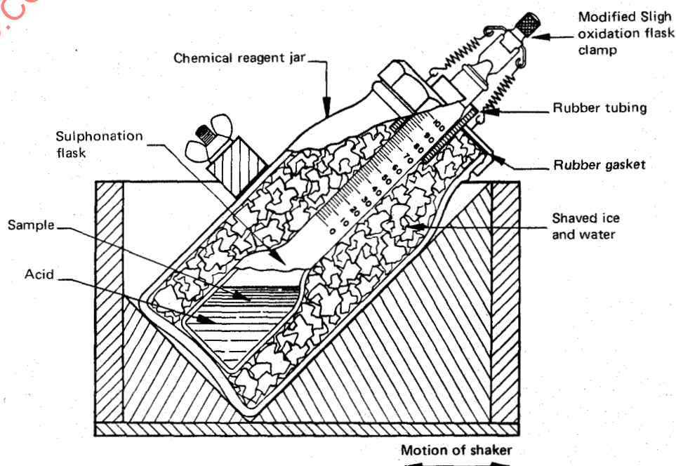
FIGURE 9 — Ice-water bath and clamp arrangement for individual sulphonation flask
