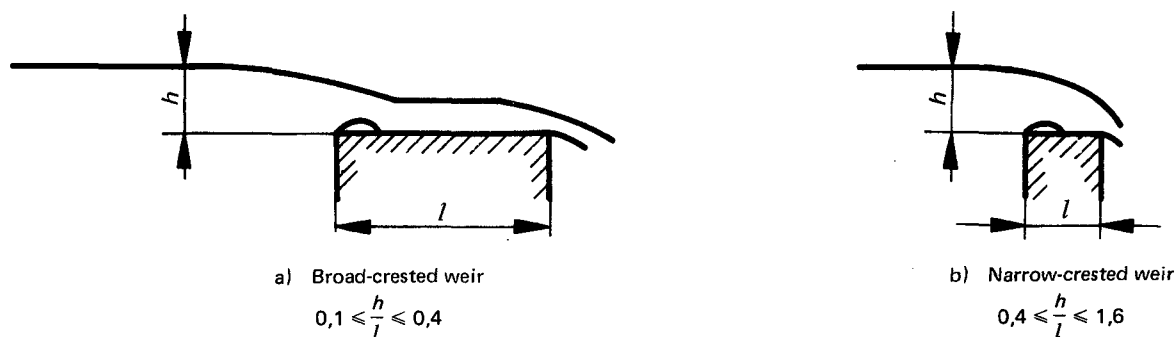
FIGURE 2 — Flow patterns over weirs of finite crest-width
