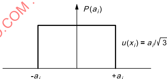
Figure C.3 — The rectangular distribution
