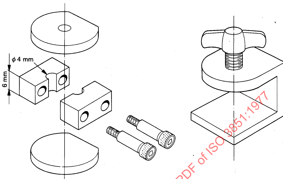
FIGURE 3 — Mould and clamp for preparation of compressive test specimen
