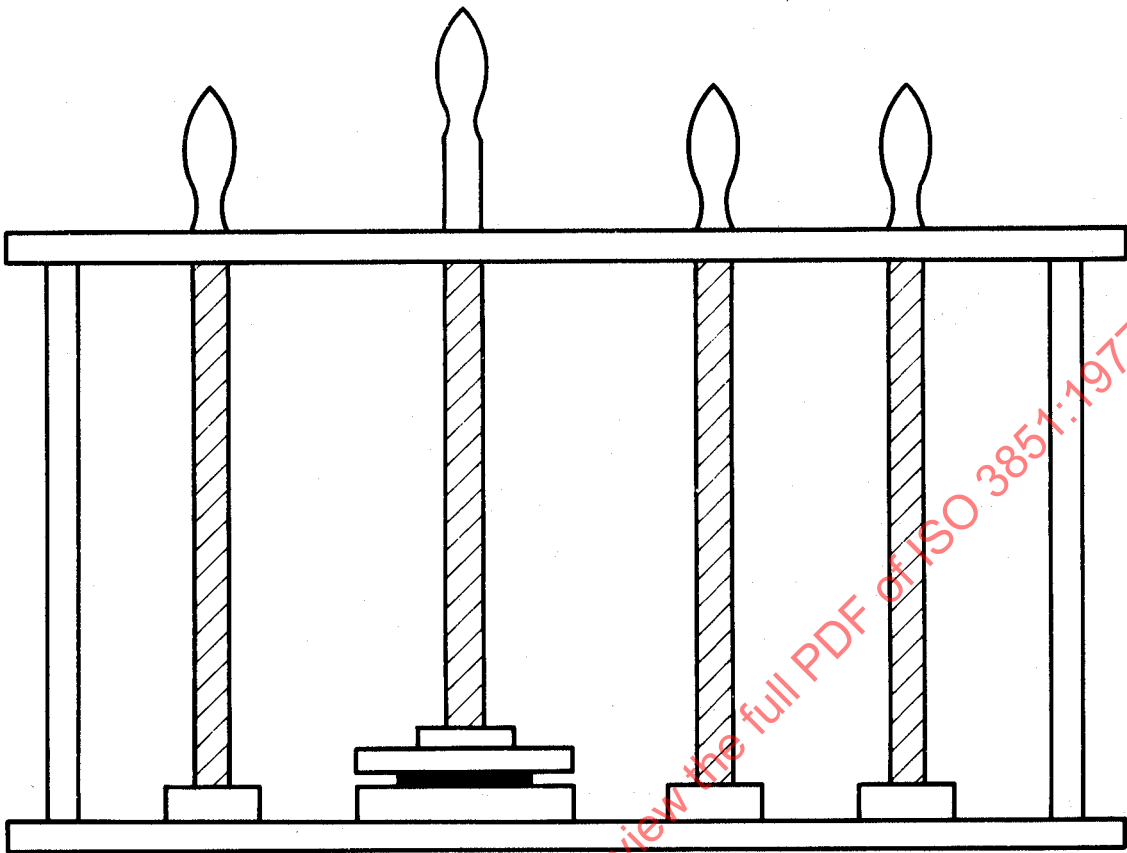
FIGURE 5 — Multiple-spring clamp
