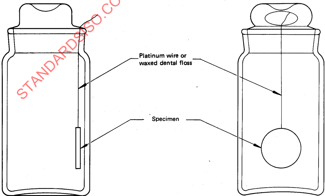
FIGURE 6 — Weighing bottle containing solubility specimen
