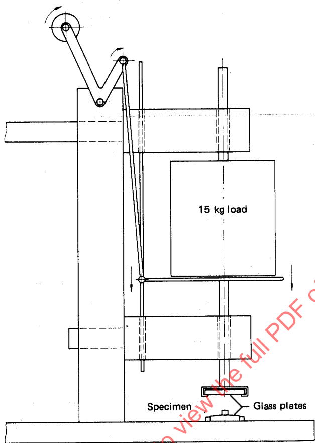
FIGURE 1 — Loading device for measuring consistency
