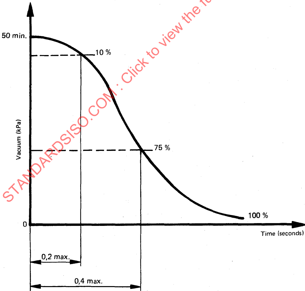
FIGURE 1 — Measurement of reaction time to the signal in the vacuum braking system from the towing vehicle to the trailer
