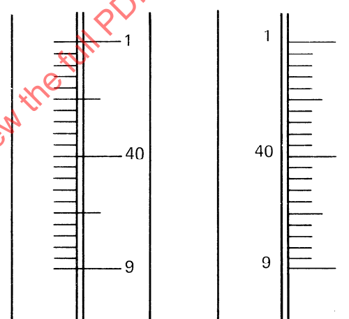
FIGURE 4 — Examples of positioning of scale lines and figuring for solid-stem thermometers
