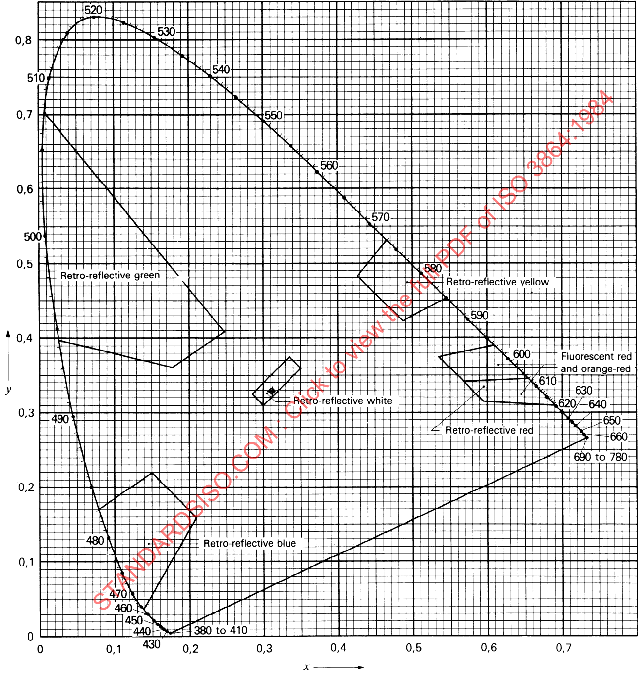
Figure 2 — Boundaries for red, yellow, green, blue and white retro-reflective surface colours and for fluorescent red and orange-red
