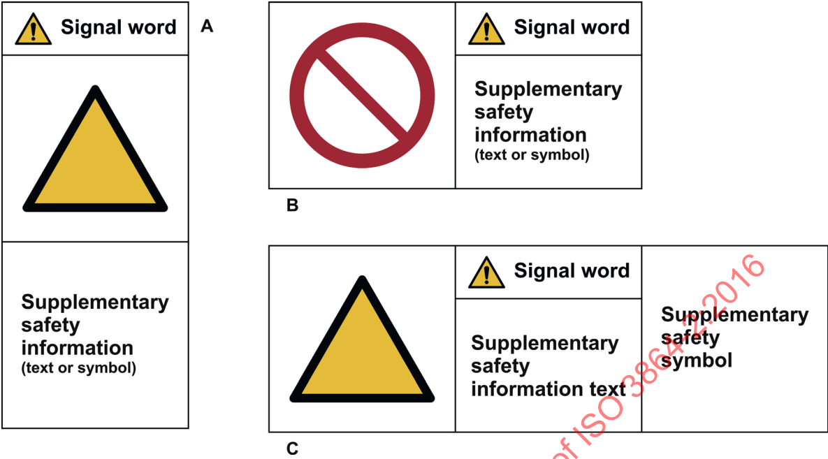
EXAMPLE A Vertical layout. EXAMPLES B and C Horizontal layout.
