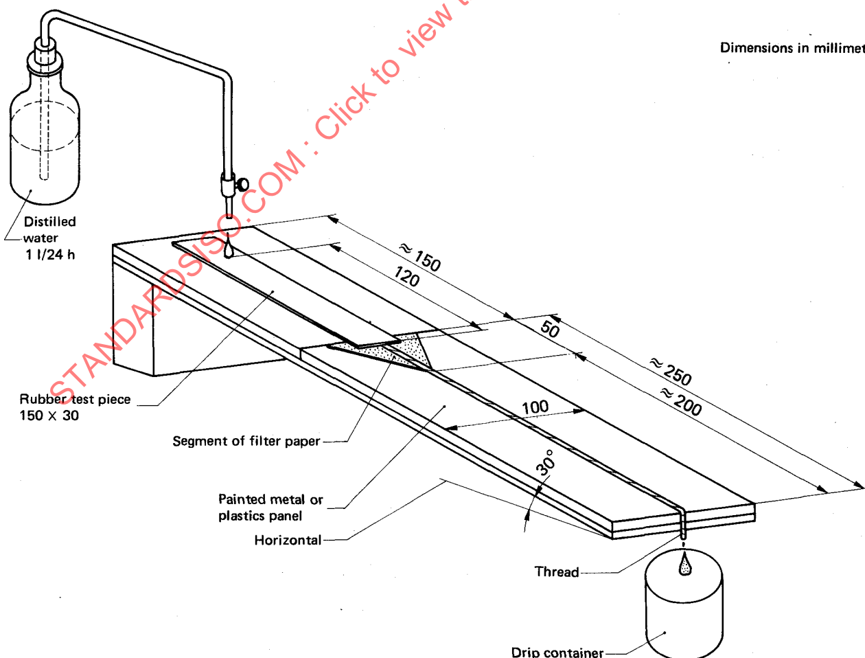
FIGURE – Dripping apparatus
