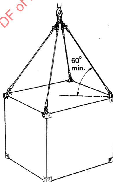
FIGURE 6 — Example of lifting containers 1D 1E and 1F
