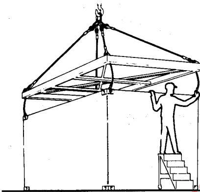
FIGURE 4a) — Attaching lifting equipment
