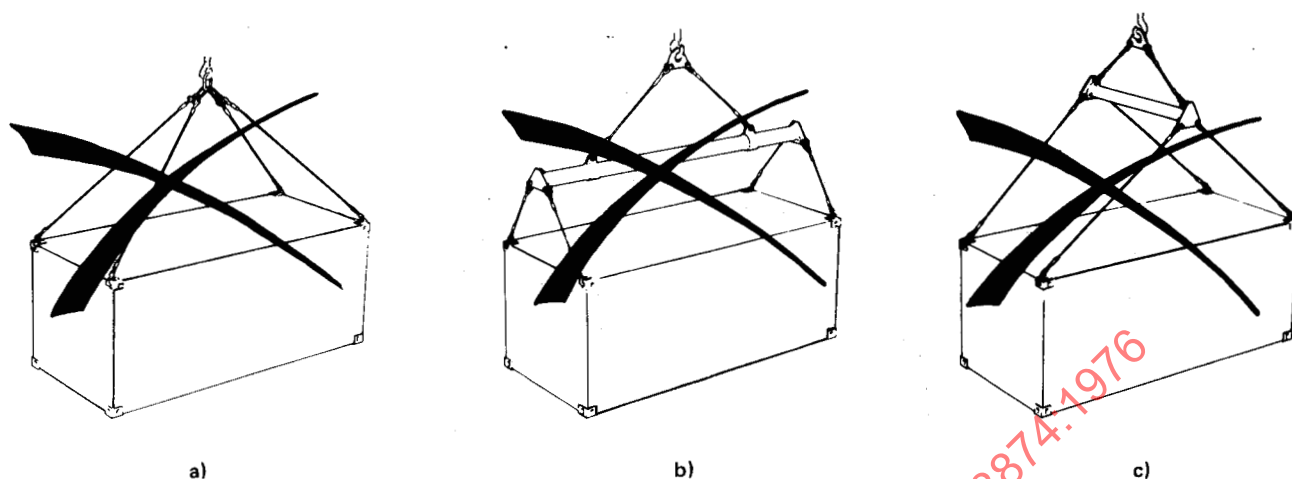
FIGURE 5 — Examples of lifting methods which must not be used
