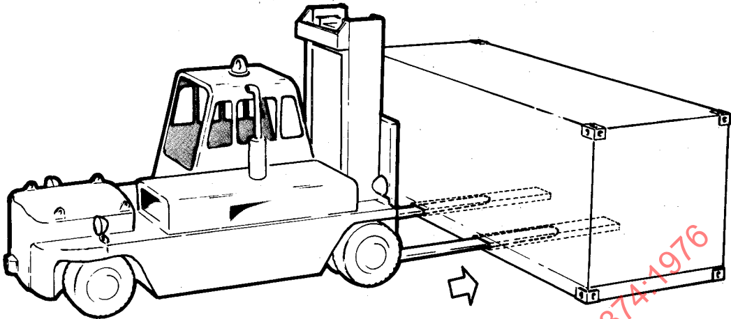
FIGURE 9 — Example of correct method of handling (with forks being inserted into or retracted from fork lift pockets)
