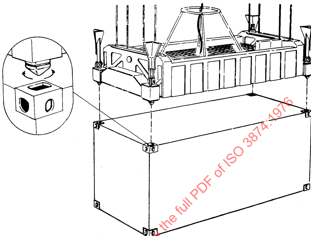
FIGURE 2 — Example of lift by crane spreader with built-in twistlocks
