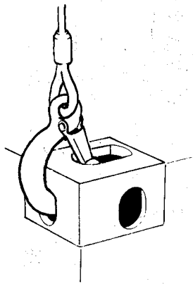
FIGURE 3c) — Example of safety hook attachment
