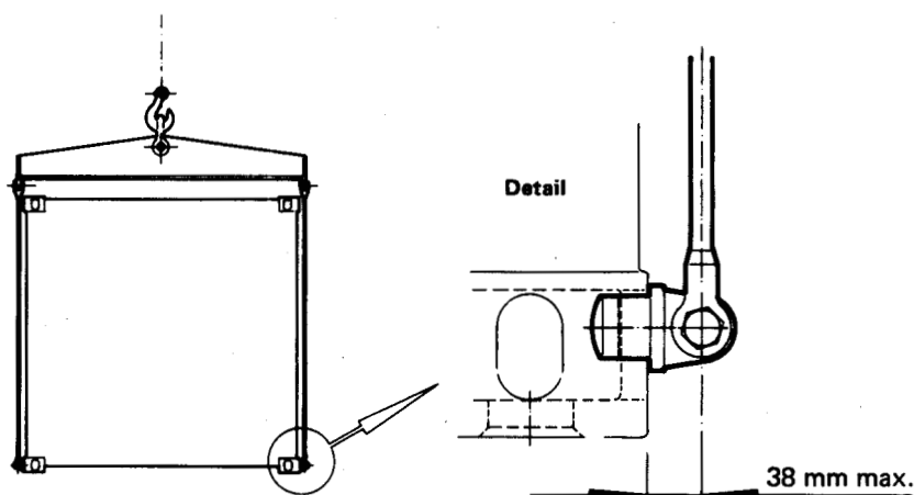
FIGURE 7 — The lifting devices should make contact with the bottom corner fittings only
