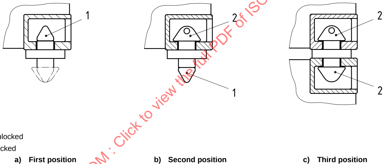
Figure A.4 — Semi-automatic twistlock, fitted to the bottom corner fitting
