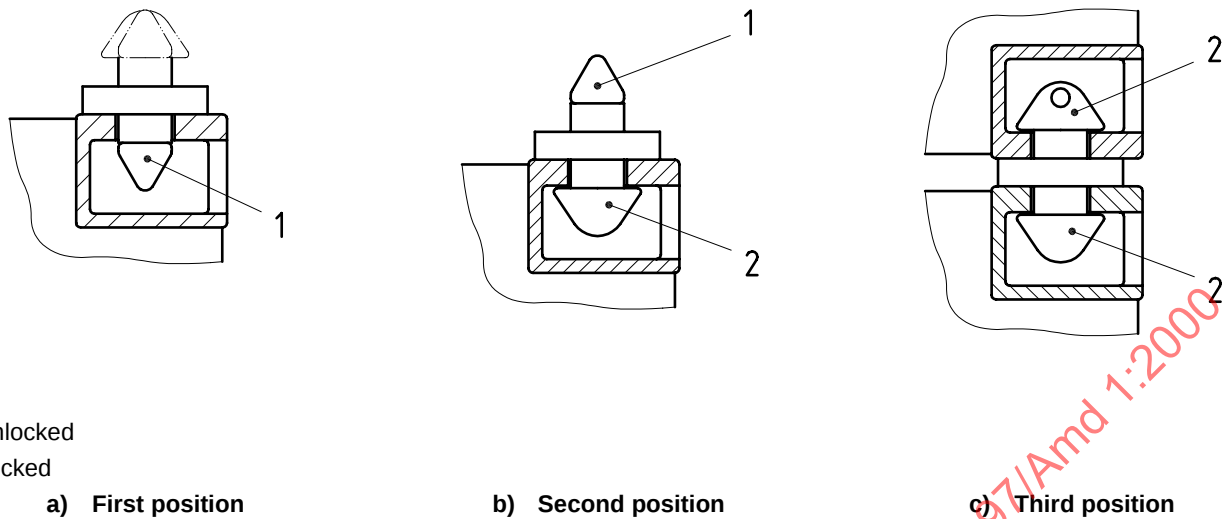
Figure A.3 — Semi-automatic twistlock, fitted to the upper corner fitting
