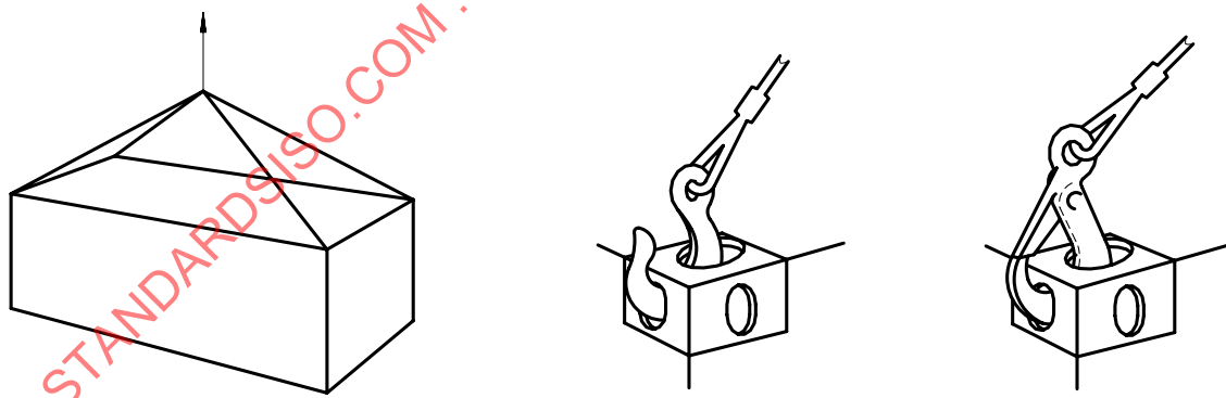
Figure 3 — Lifting by means of a top lift sling
