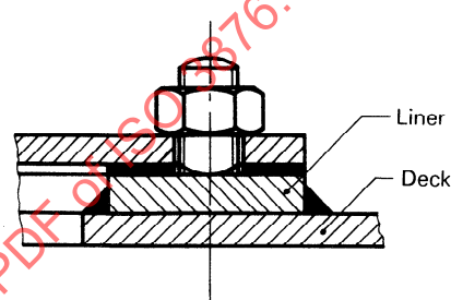
Figure 9 — Inside welding on deck
