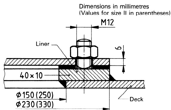
Figure 2 — Type B (hand-hole without coaming)
