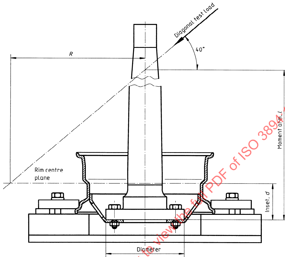
Figure 2 — Dynamic cornering fatigue test — 40° loading method
