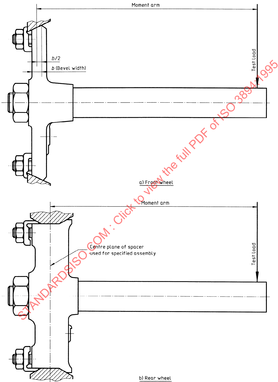
Figure 3 — Wheels with demountable rims — Dynamic cornering fatigue test
