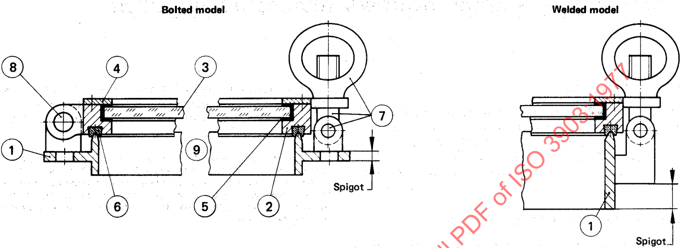
FIGURE 3 – Opening window
