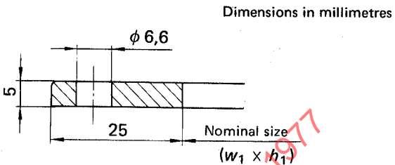
FIGURE 13 – Glass retaining frame, minimum dimensions
