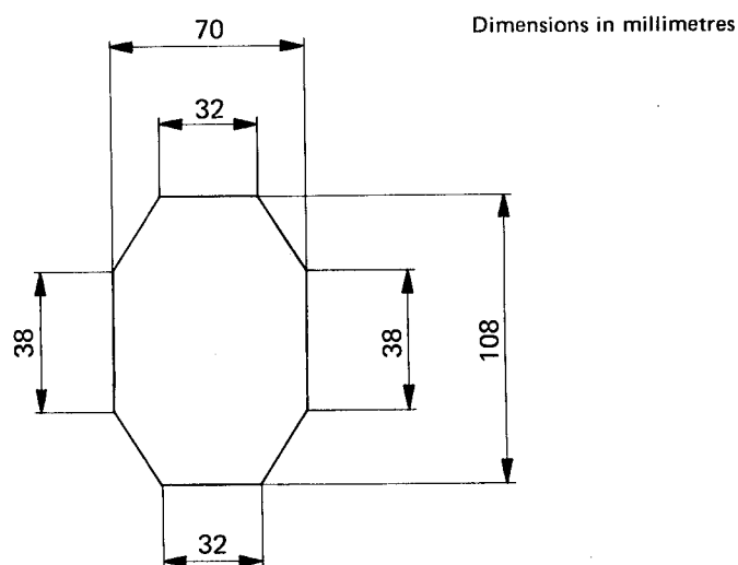
FIGURE 2 — Test piece for flexing test
