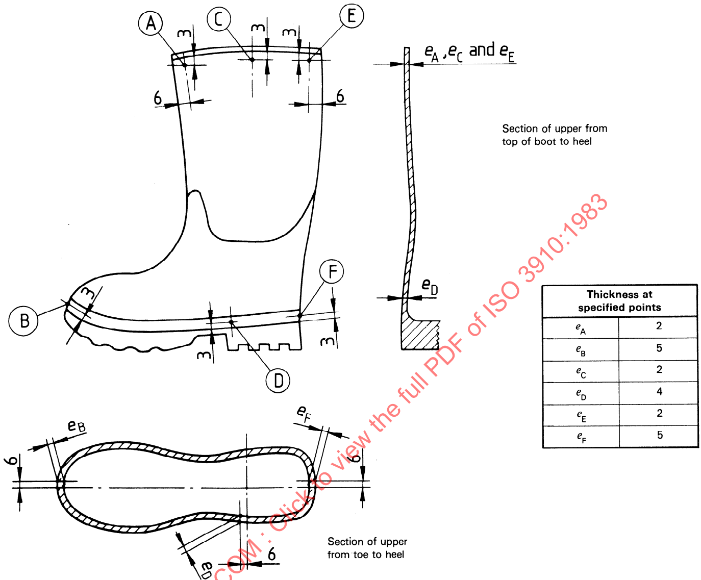
Figure 1 — Unlined moulded rubber boot
