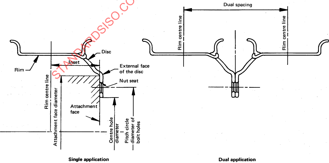
FIGURE 2 — Truck disc wheel nomenclature
