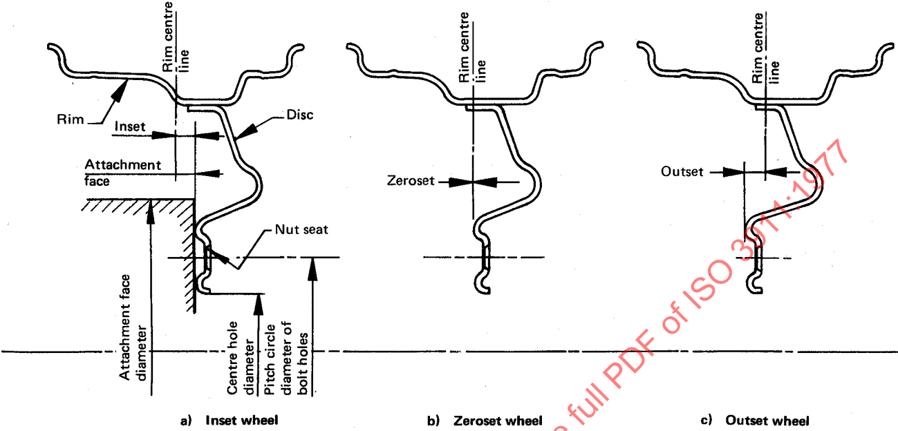
FIGURE 1 — Passenger car and light truck disc wheel nomenclature
