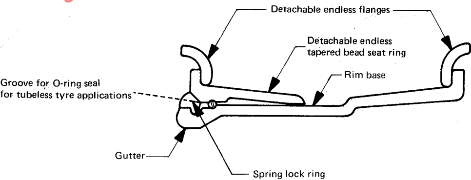
FIGURE 13 – Five-piece rim nomenclature
