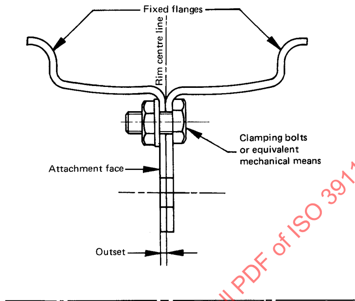
FIGURE 3 – Divided wheel nomenclature
