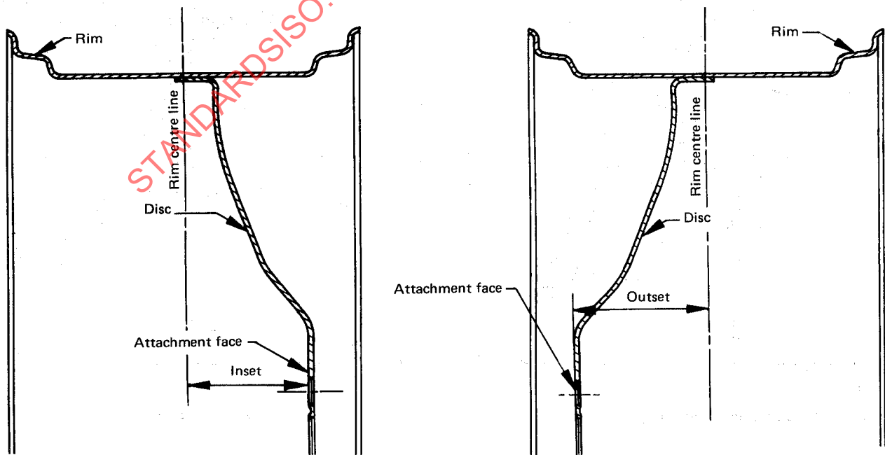
FIGURE 6 – Reversible wheel
