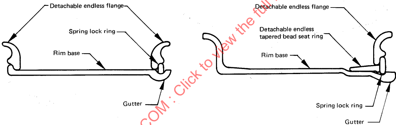
FIGURE 12 – Four-piece rim nomenclature
