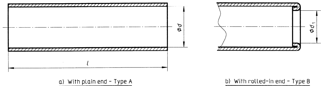
Figure 1 — Cylindrical tubes
