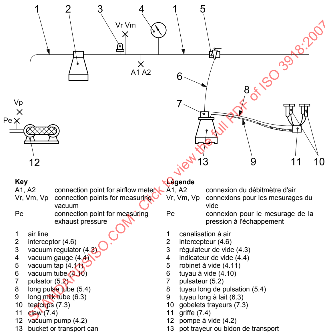
Figure 1 — Example of bucket or direct-to-can milking machine
