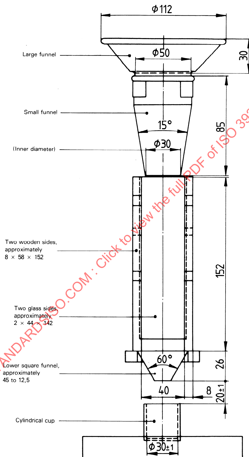
Figure 1 — Test apparatus — Front view
