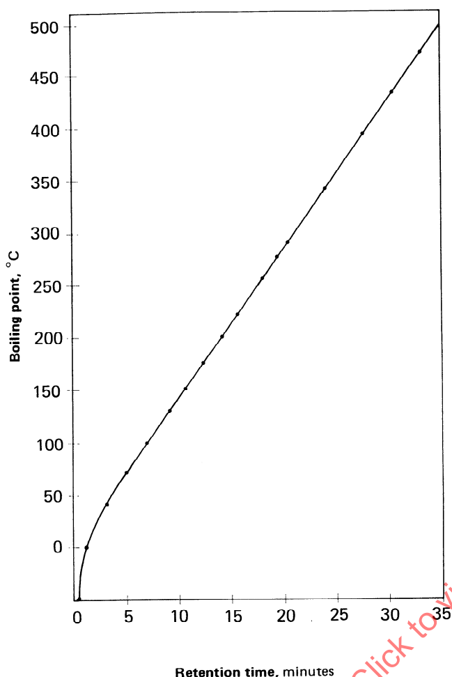
FIGURE 2 — Calibration curve
