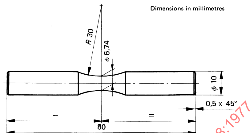
FIGURE 3 — Schenck test piece
