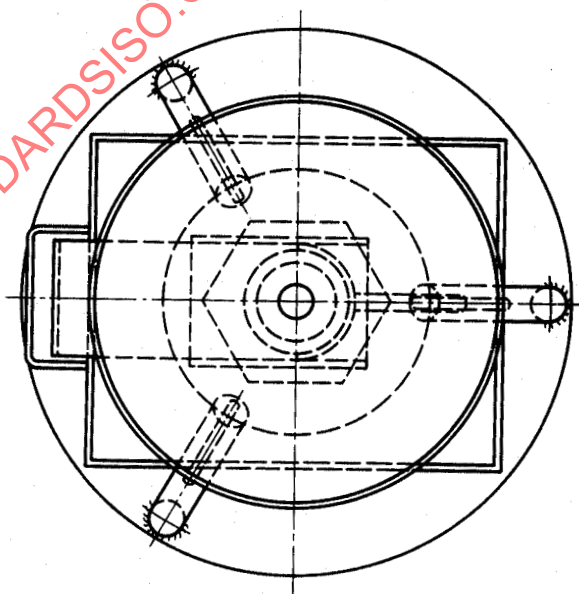
Figure — Apparatus for the determination of bulk density of fertilizers
