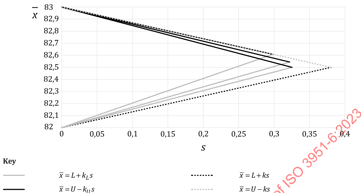
Figure H.2 — acceptance region, s -method, combined control – construction lines
