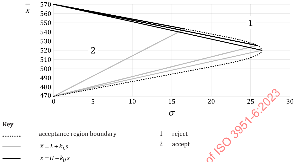
Figure H.6 — acceptance region, \sigma -method, combined control with construction lines
