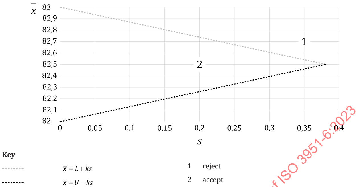
Figure H.1 — acceptance region, s-method, separate control
