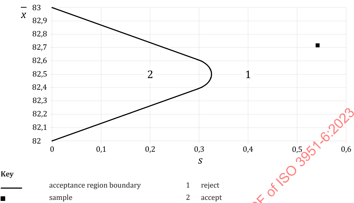
Figure 3 — Example of the use of an acceptance diagram, s-method
