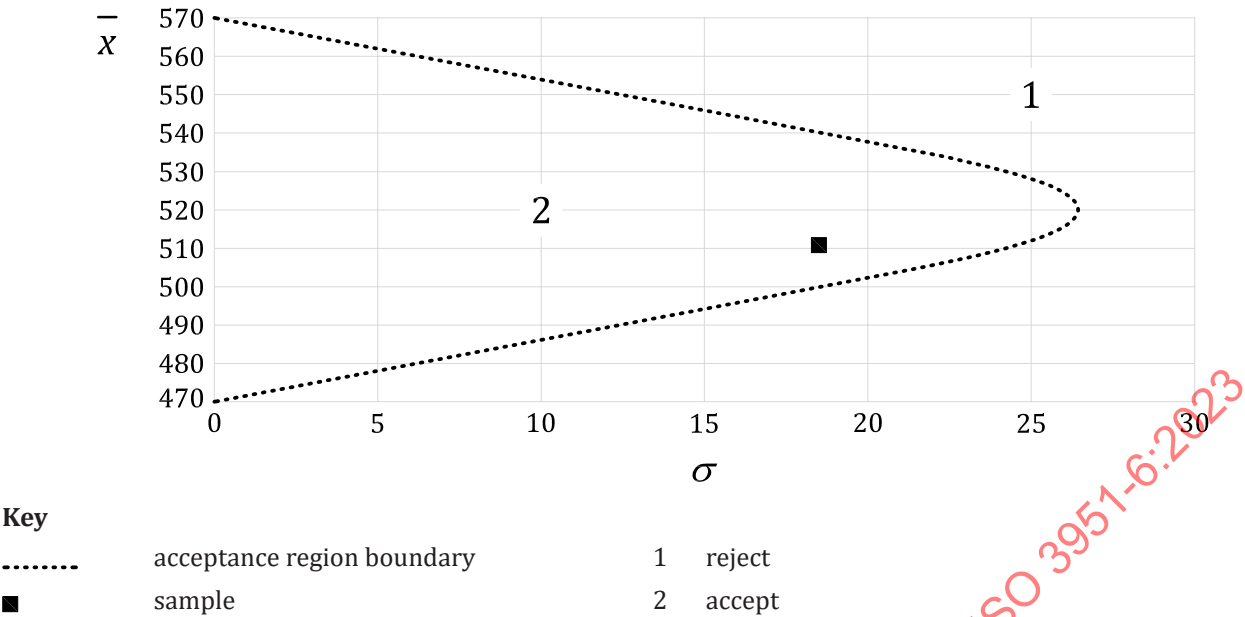
Figure H.7 — Acceptance region, \sigma -method, combined control with sample mean and standard deviation
