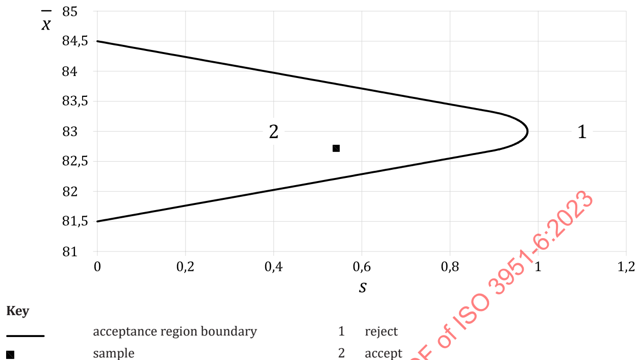
Figure 4 — Example of the use of a combined control double specification limits acceptance diagram, s-method
