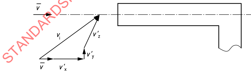
Figure C.1 — Pressure probe insensitive to orientation
