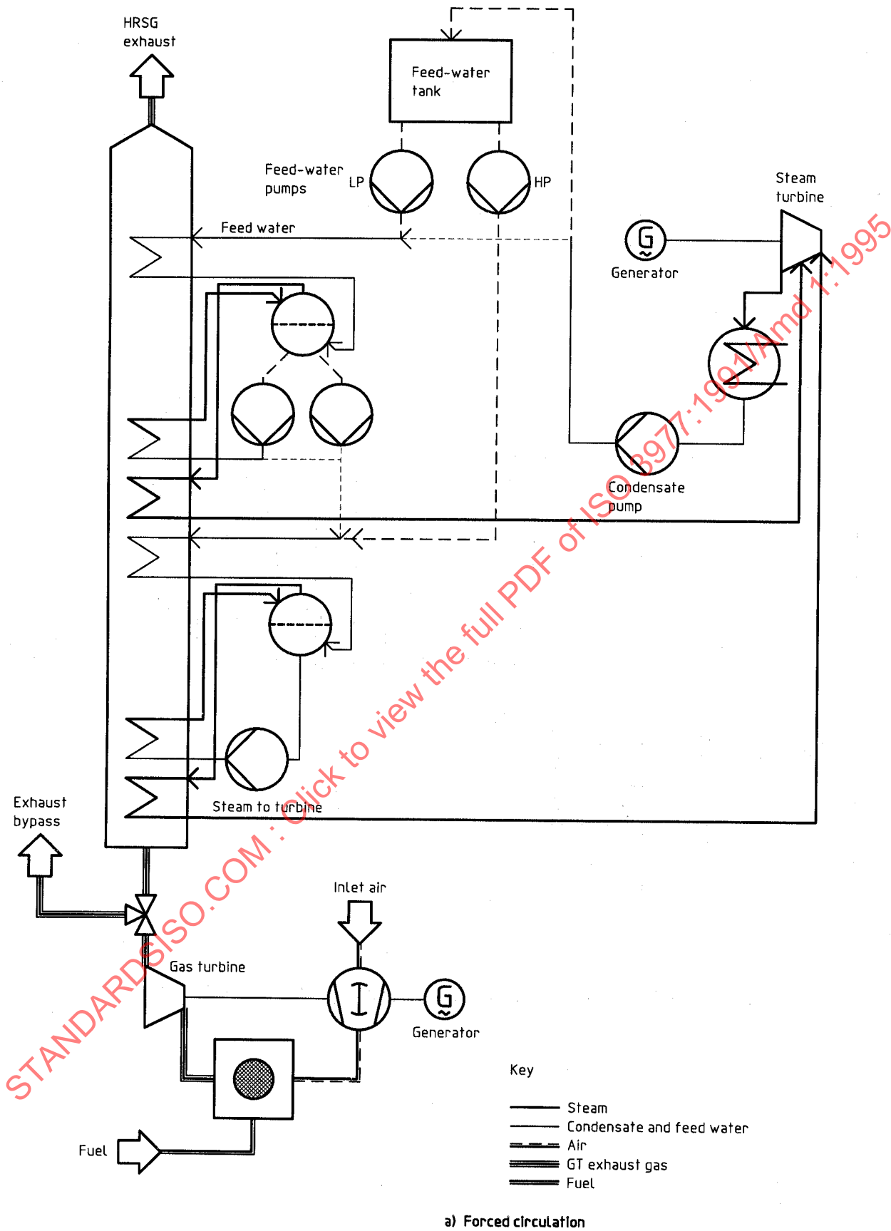
Figure C.6 — Equipment/cycle options: multi-pressure combined cycle — Two-pressure HRSG
