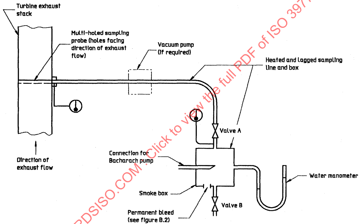
Figure B.1 — Schematic illustration of smoke spot smoke sampling system
